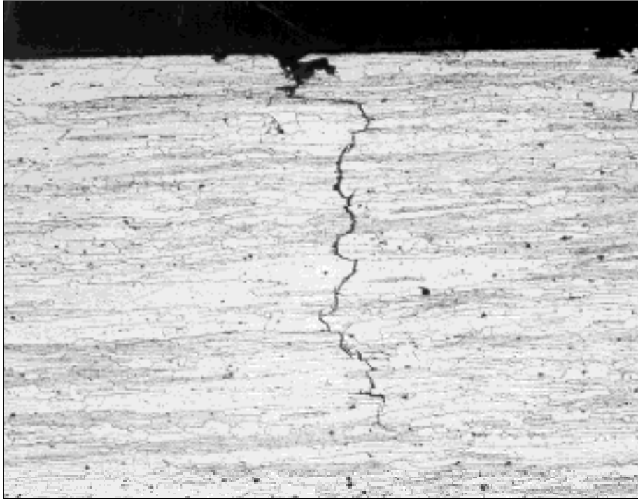
Figure 1 Transcrystalline stress-corrosion cracking revealed by metallographic analysis carried out on a 7449-T651 aluminium alloy sample tested for SCC susceptibility. The crack initiated from a corrosion pit formed during exposure to 3.5 % NaCl water solution (Mag. X100).
