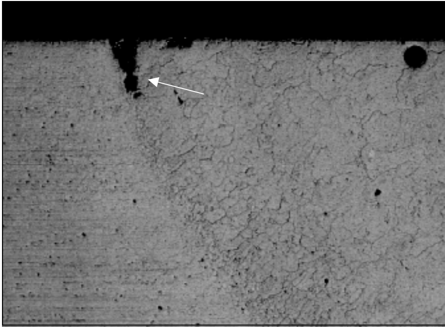
Figure 5 Example of pitting corrosion damage in a MIG welded 7020-T6 aluminium alloy tested for stress-corrosion cracking. A corrosion pit, visible in the photo, in the region of transition between the fused zone and the parent plate. No evidence of SCC was found (Mag. X50).
