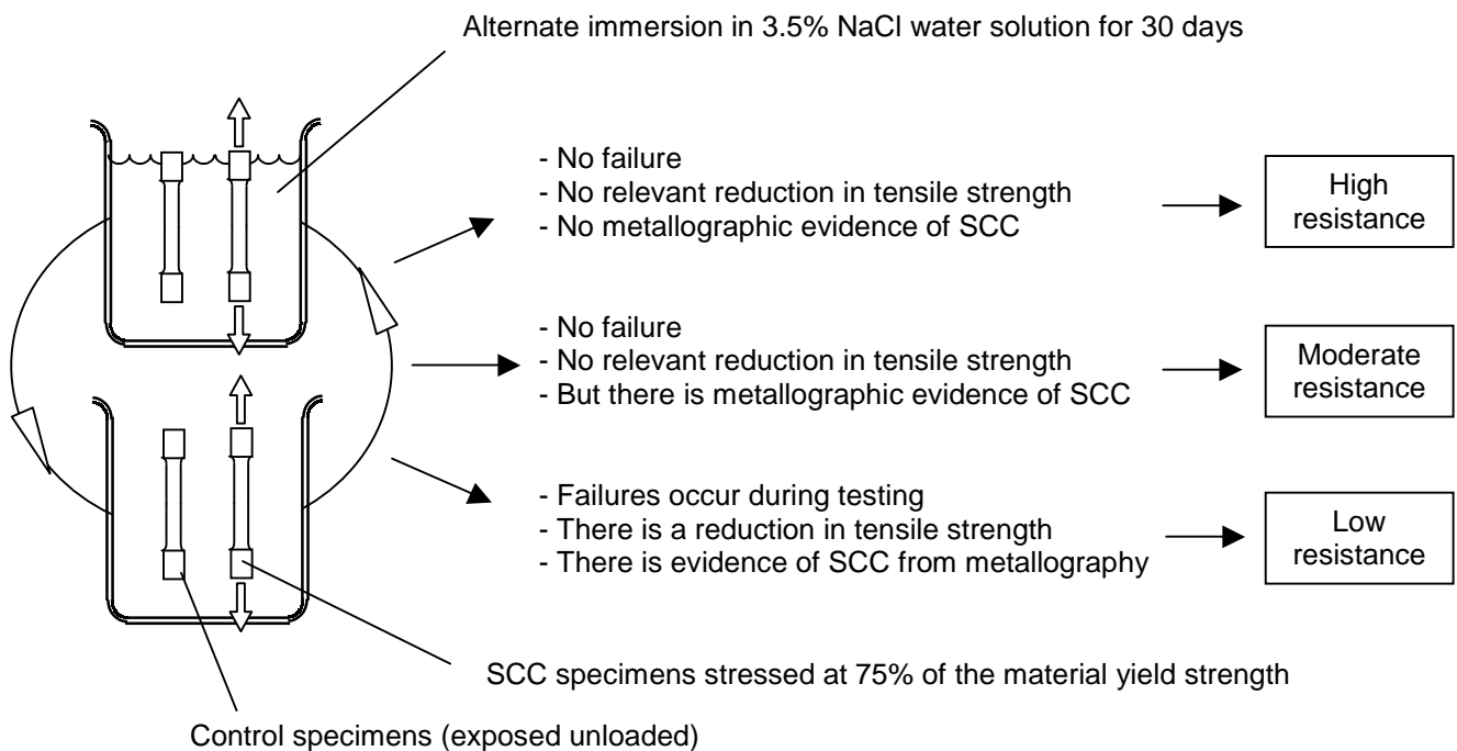
Figure 4 Representation of the constant load SCC test procedure and interpretation of results.
