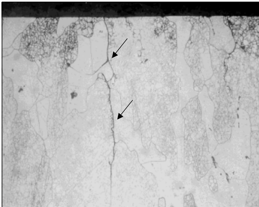
Figure 2 Example of intergranular stress-corrosion cracking in a 7075-T651 aluminium alloy tested in accordance with the constant load method ECSS-Q-70-37 (Mag. X200).
