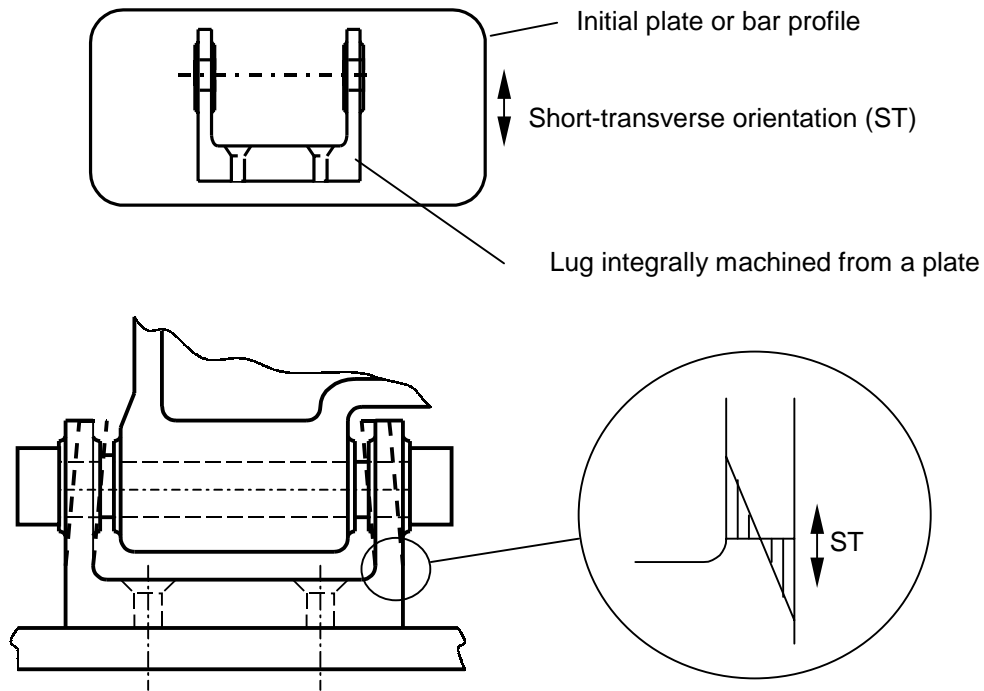
Figure 3 A typical case where sustained stresses are introduced into the component during assembly. SCC can be prevented by modifying the manufacturing process - to change the grain orientation with respect to the direction of sustained tensile stress - and the design - to reduce the clearance between lugs. An alloy/heat treatment highly resistant to SCC should be selected for this application.
