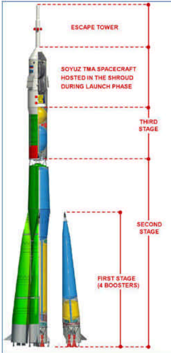
Artist's Impression of Soyuz FG launcher (Image: G. De Chiara Mars Center/2002)
