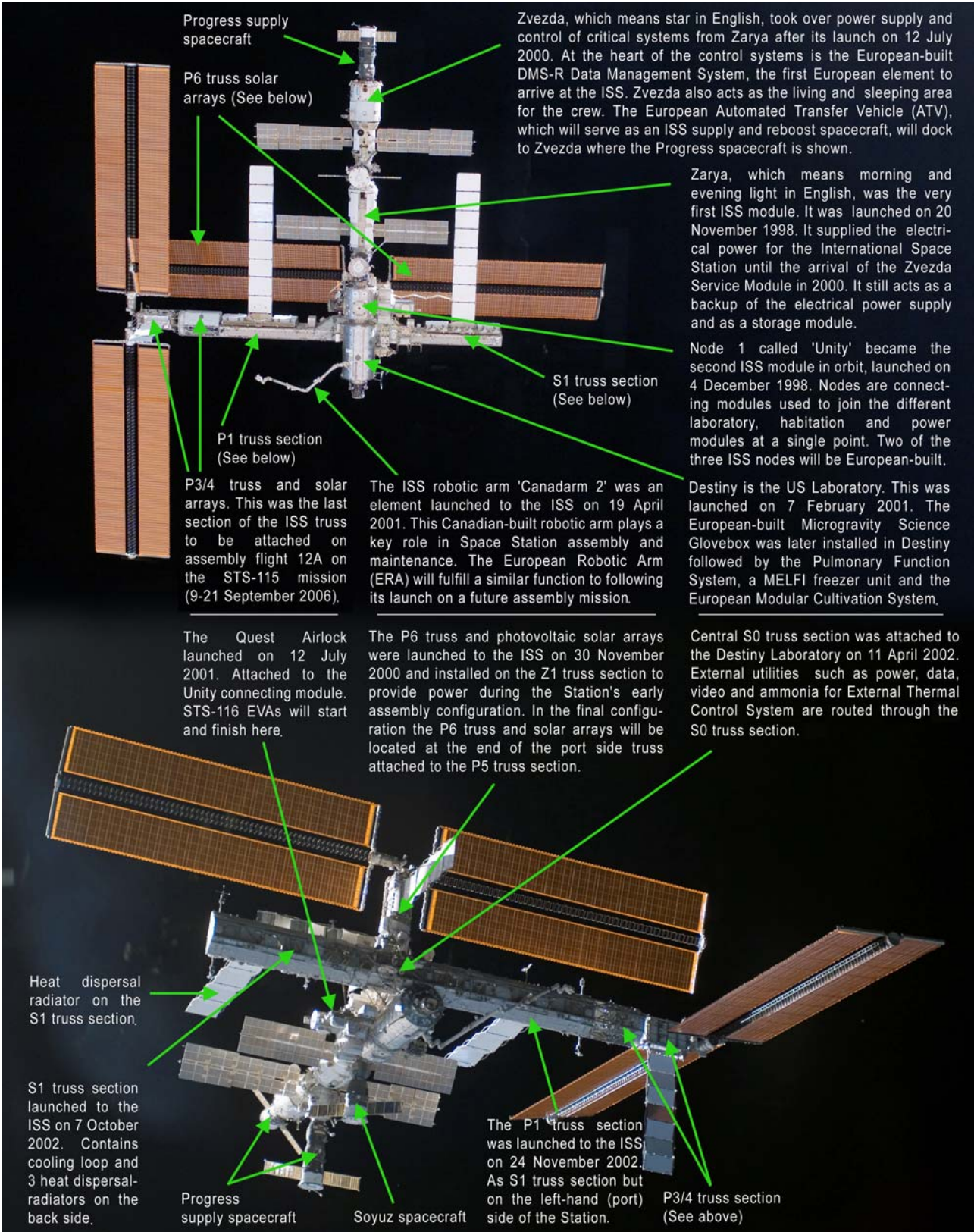
ISS Current Configuration: (Top) Underside or Earth-facing view of ISS. (Bottom) Front/Earth-facing side of ISS (Image: NASA/Text: ESA)
