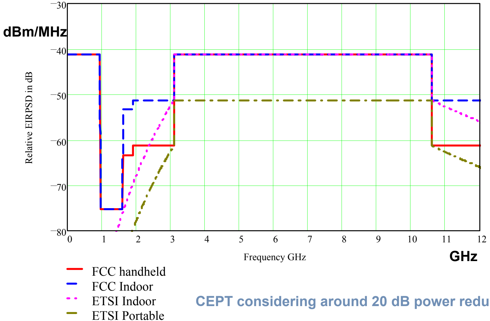
FCC and ETSI radiated power masks
